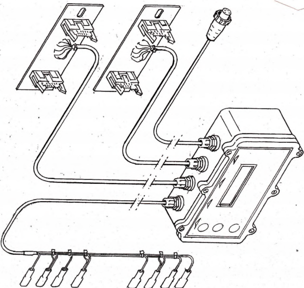
4101-300 AB CONTROL ELECTRONICS ASSY
