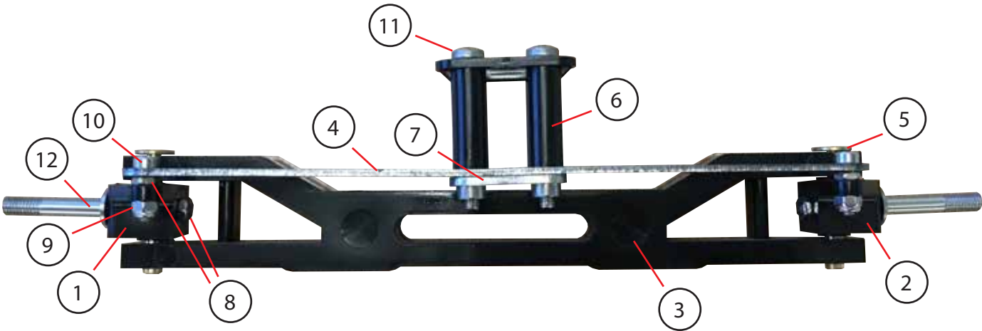
5J00-452 - Steering assembly 1/8
